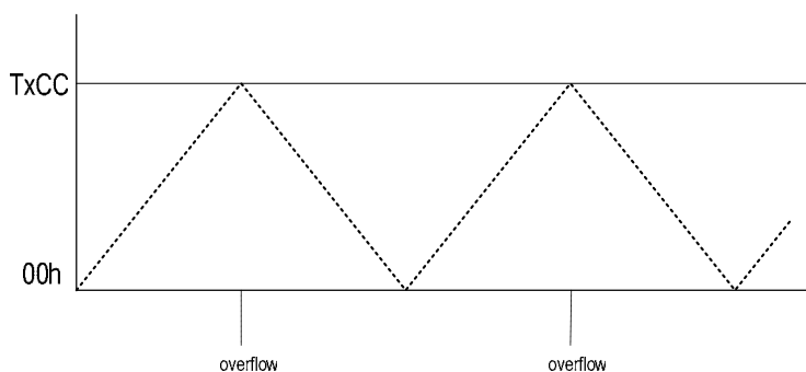
Figure 24 Up/down Mode
