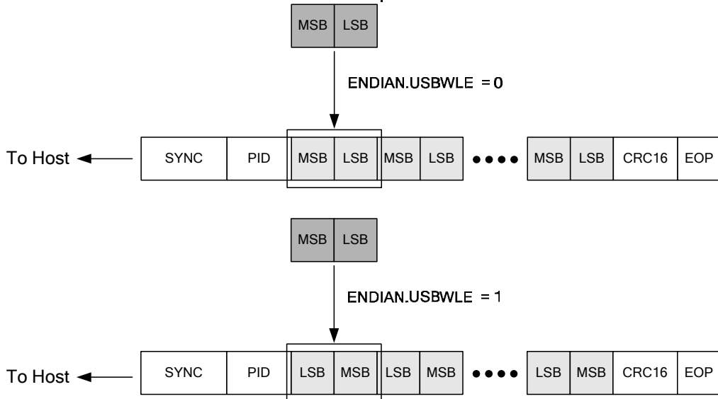
Figure 37 Writing Little/Big Endian
